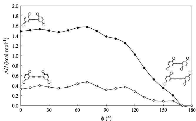
Figure 3. Potential energy curves for the \text{--C}\equiv\text{C--} ( QAAQ , filled circles) and \equiv\text{C--C}\equiv ( QAAQ , open circles) bond rotation relative to the energy of the conformers ( \phi=180^\circ ) calculated by B3LYP/6-311+G(d,p) methods.
