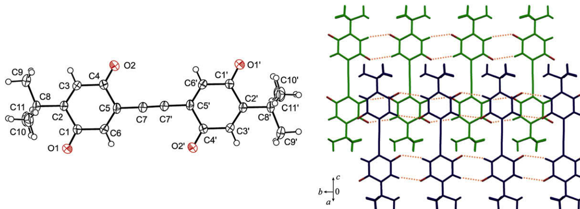
Figure 1. X-ray structure of QAQ . (left) ORTEP drawing (50% probability). (right) A top view of ribbon motif formed by CH/O interactions (represented by orange broken lines).
