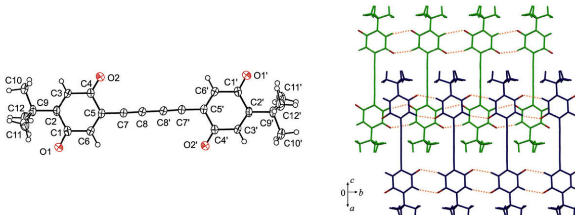
Figure 2. X-ray structure of QAAQ . (left) ORTEP drawing (50% probability). (right) A top view of ribbon motif formed by CH/O interactions (represented by orange broken lines).
