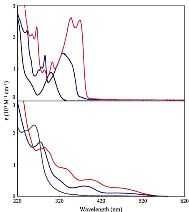
Figure 4. Electronic absorption spectra of MM (upper black), MAM (upper blue), MAAM (upper red), QQ (lower black), QAQ (lower blue), and QAAQ (lower red) in 1,4-dioxane.
